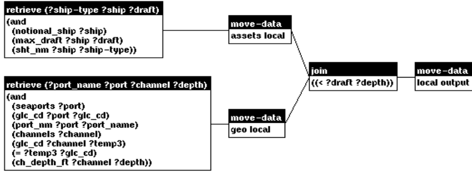
Figure 5: Parallel Query Access Plan
