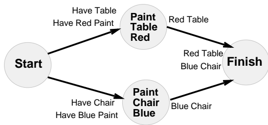
Figure 1: Plan With Independent Actions
