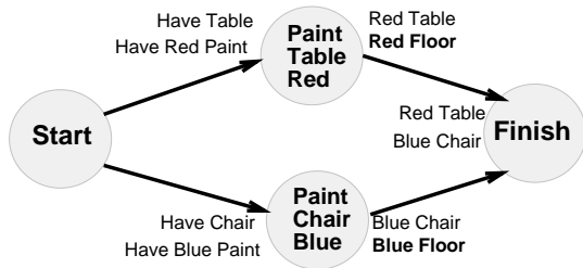
Figure 2: Plan with Independent Actions Relative to the Goal
